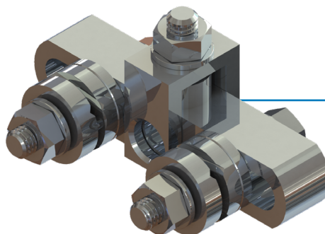
Conector barra-barra-pino Pin bar bar connector
